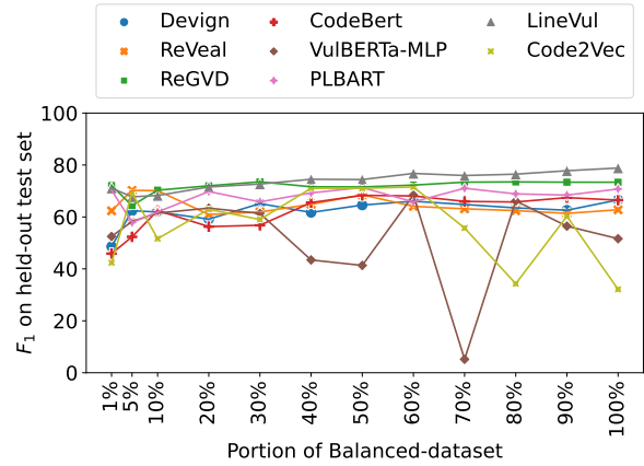
(a) Results on Balanced-dataset. 100% dataset size = 45,363.
