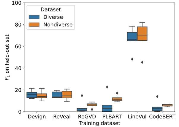
(a) Diverse vs. non-diverse performance
