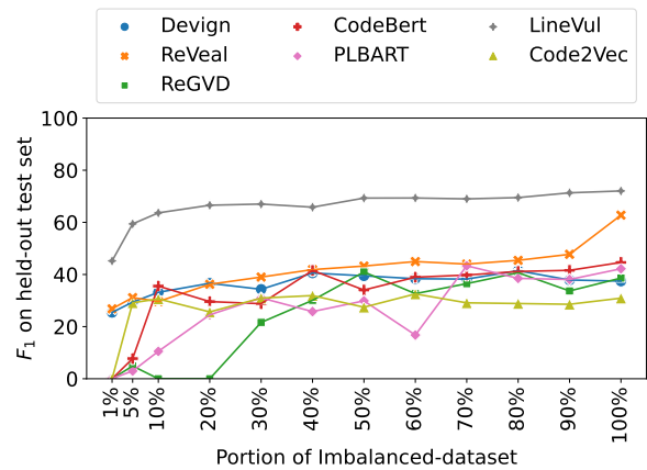
(b) Results on Imbalanced-dataset. 100% dataset size = 194,285.
