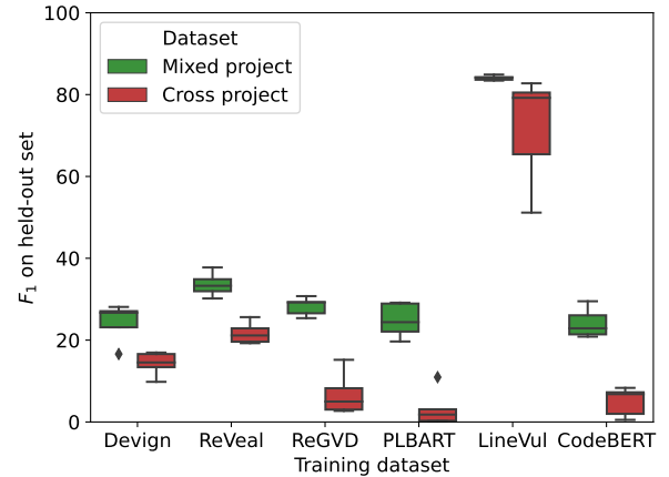
(b) Mixed-project vs. cross-project performance
